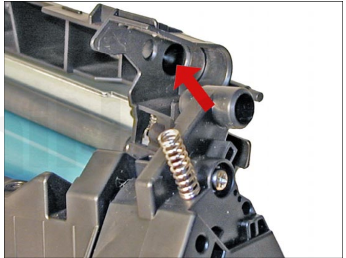
25. Place the drum/waste hopper into the toner hopper.
