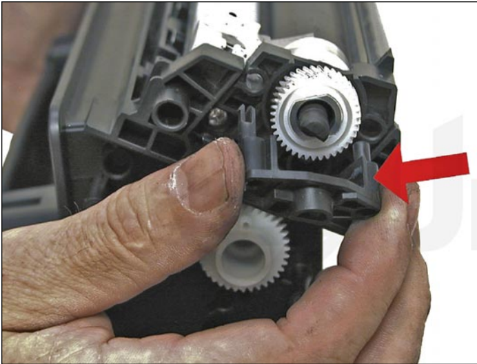
19. On the supply chamber, carefully pry off the magnetic roller sleeve cover, and remove.
