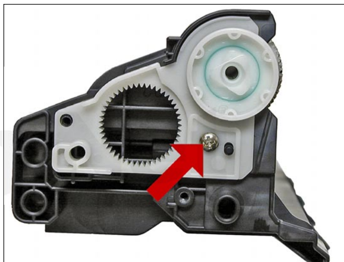
8. On the large gear side of the waste chamber, remove the screw and white plastic drum bushing.
