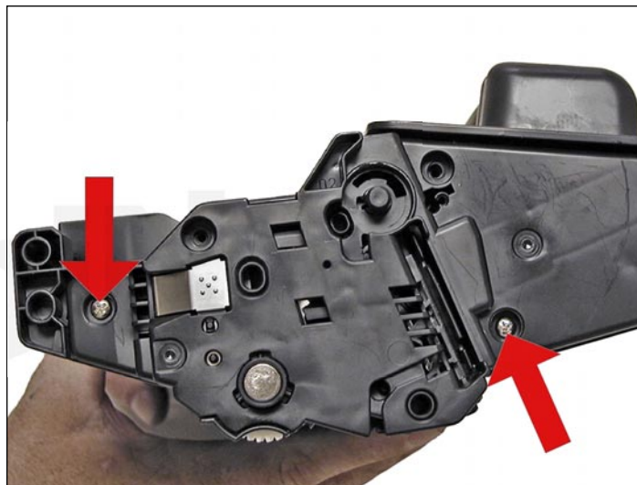
37. Hold the two sections of the cartridge together, and install the left (contact side) end cap. Install a screw in the waste and supply sections to hold everything together.
