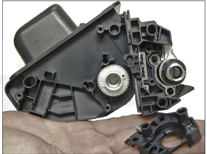
22. Remove the two screws, spring, and the holder.
