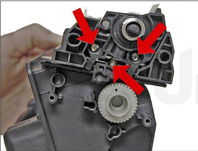
21. Note the location of the spring between the magnetic roller sleeve holder and the hopper.
