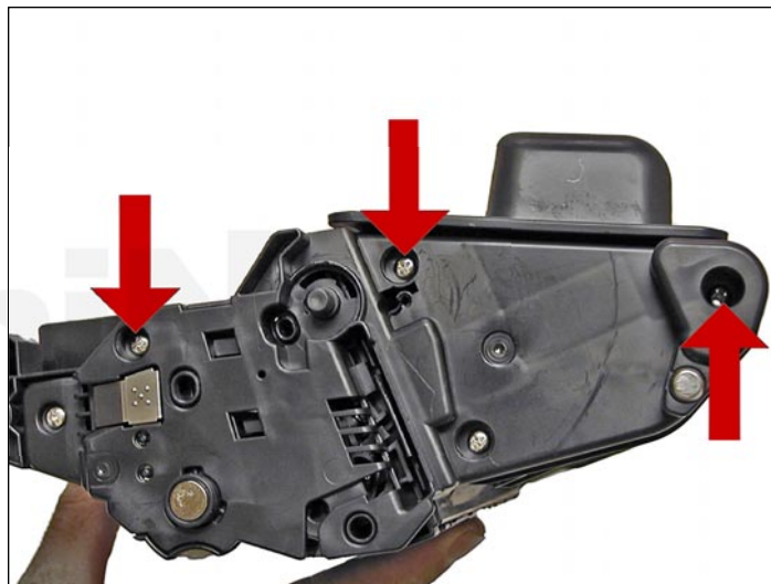
39. Install the remaining three screws on the left end cap.
