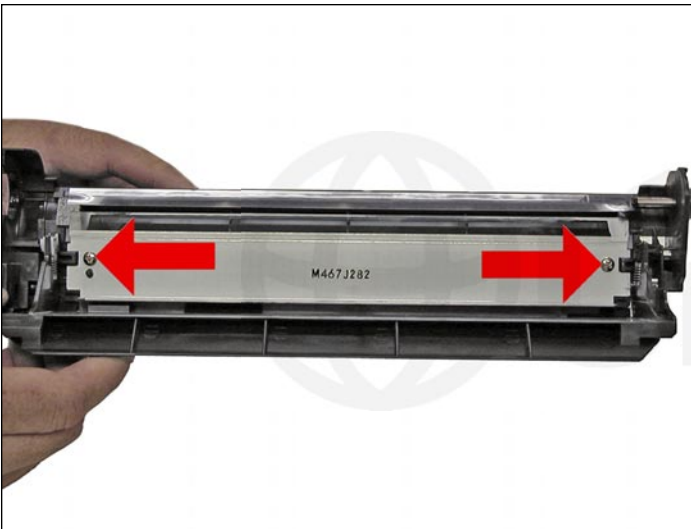
11. Remove the two screws from the wiper blade.
