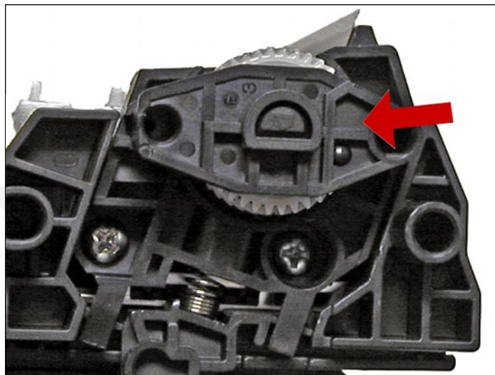
35. Install the keyed magnetic roller sleeve cover. Make sure that the keyed hole in the cover matches the keyed end of the magnet in the magnetic roller sleeve assembly.
