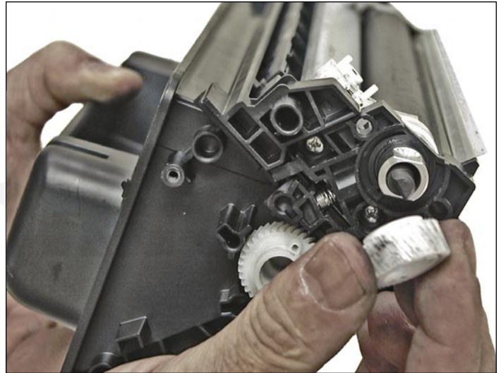
20. Remove the magnetic roller sleeve drive gear.
