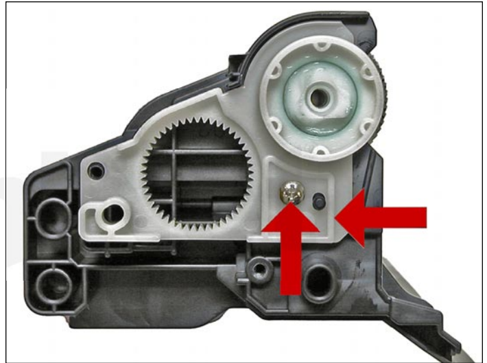
18. Install the white plastic drum bushing and screw. If the OEM drum grease is dirty, clean it off with alcohol, and replace with white lithium grease.
