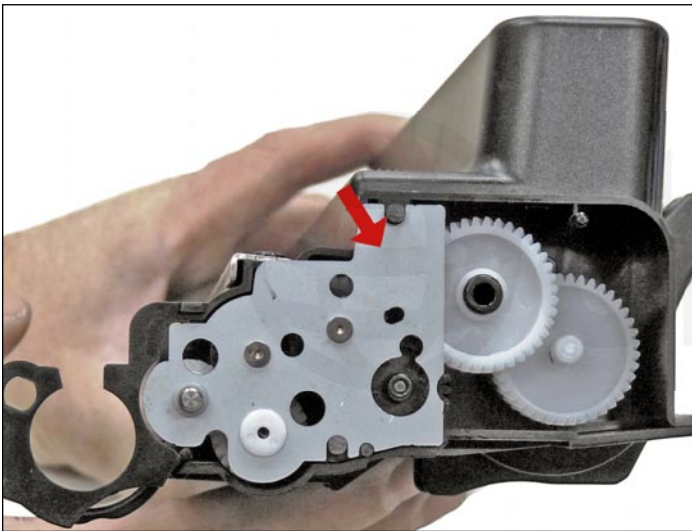
23. Pry off the gear plate, and remove the gears.
