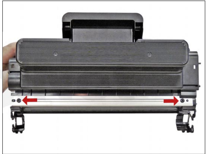
26. Remove the two screws from the doctor blade, and remove the blade. Clean out all the remaining toner from the hopper.
