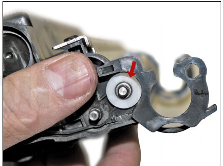
24. Remove the developer roller bushings from both sides.
