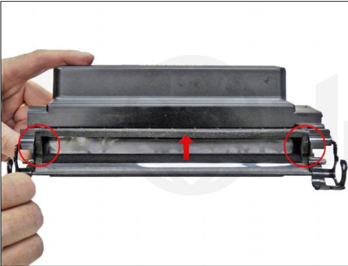
27. Make sure the doctor blade sealing foam and the developer roller seals are clean and intact.
