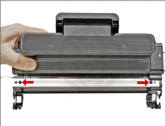
31. Install the doctor blade and two screws.
