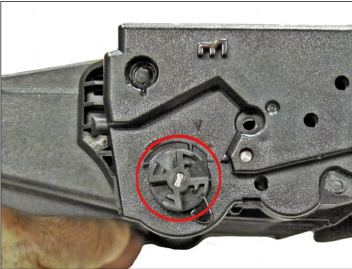
44. Install the drum drive gear.
