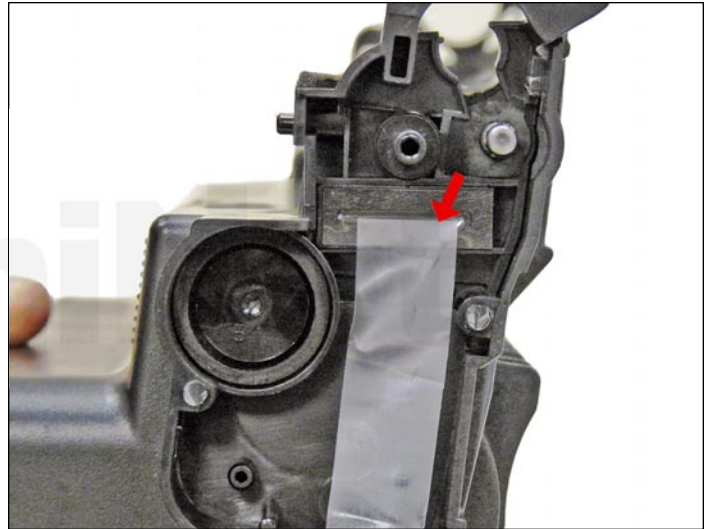
30. Pull the tail of the seal through the seal port.
