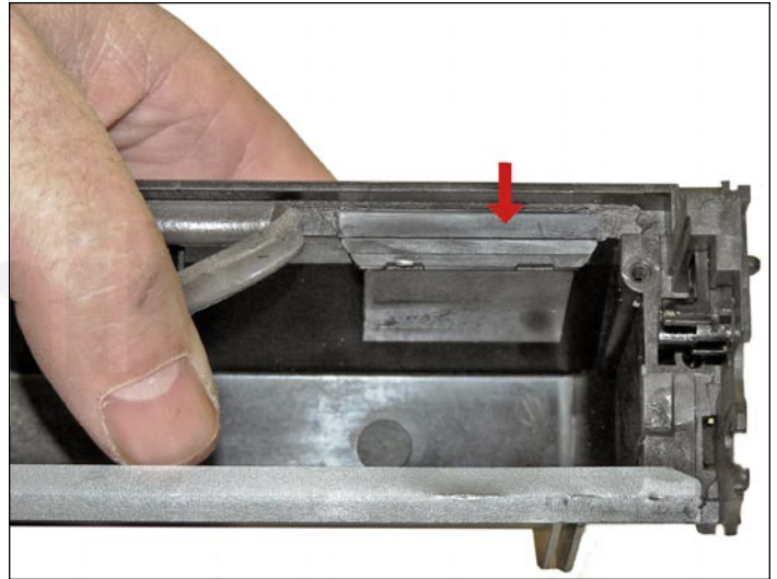
17. Replace the chip cover.
