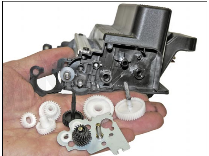
23. Pry off the gear plate, and remove the gears.
