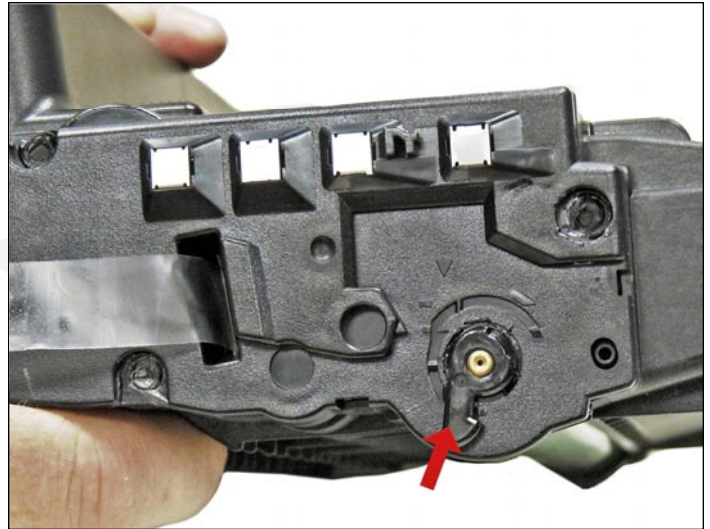
45. The drum separators are fixed to the end caps. They should be set as shown. These arms keep the drum and developer rollers separated until the cartridge is installed in the printer.
