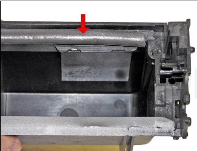
18. Reinstall the wiper blade seal. Use 100% silicon if the seal is torn to prevent any leaks. Just as the OEM did, be careful not to use any silicon on the chip cover area (otherwise it will be very difficult to replace the chip on the next cycle).
